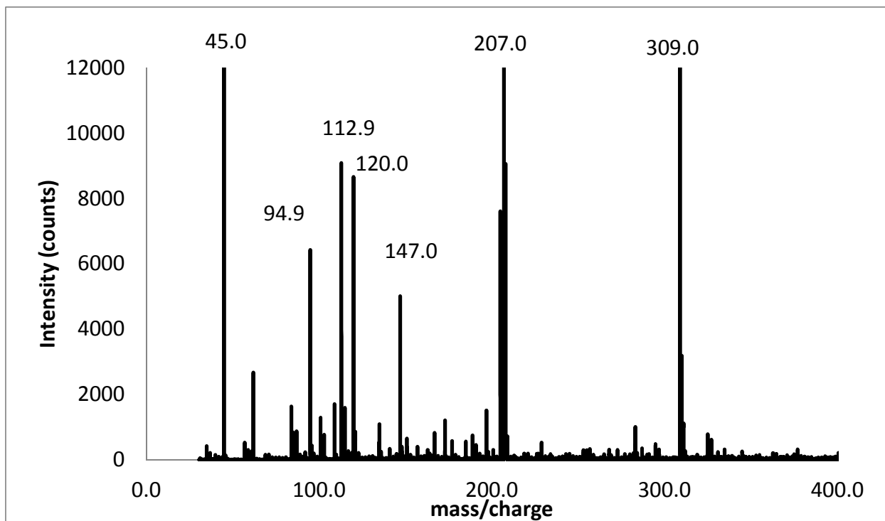
Figure S2. Full range mass spectrum of sodium reduced PP in THF solution measured at a retention time of about 8 minutes.
