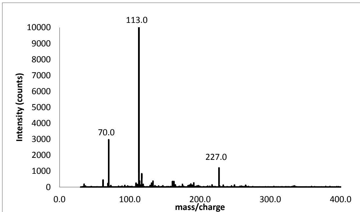
Figure S1. Full range mass spectrum of sodium reduced PP in THF solution measured at a retention time of about 2 minutes.
