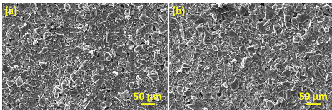
Figure S1. SEM microstructures; (a) before GCD and (b) after 5000 GCD cycles at 3.75 \text{ A g}^{-1} of CAR 900 electrode.
