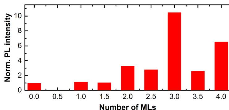
Figure SI8. PL evolution of the CdSe/ZnS/CdS3 NCs as a function of the shell thickness: initial PL intensity value remained almost unaltered after ZnS layer deposition and then increased six-fold of the starting value (the numbers are normalized areas under PL curves plotted on energy scale).
