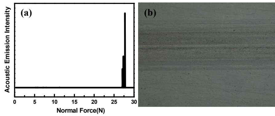
S1 SiO 2 -MgF 2 double coatings' mechanical properties. (a) Acoustic emission spectrum of scratches between the coatings and the substrate. (b) Scratches by 6 H pencil on the surface of the coatings.
