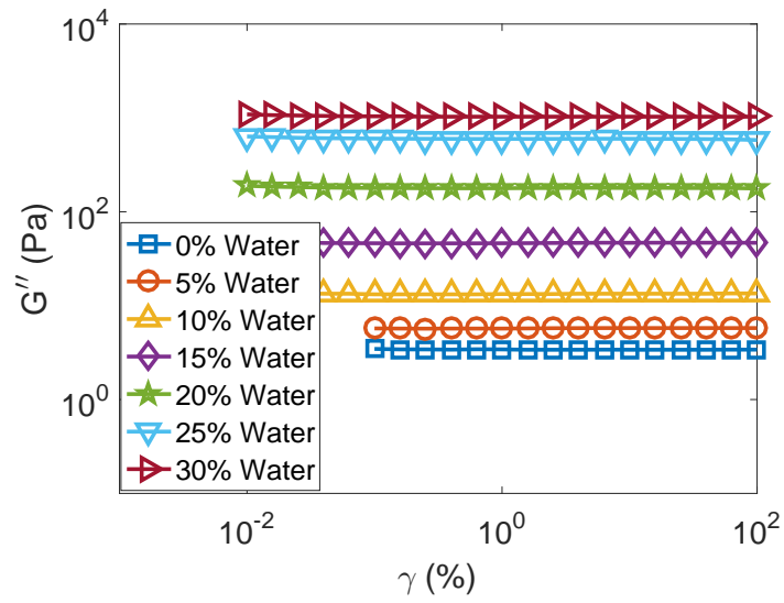
Figure 2: Determination of linear viscoelastic regime in hA/QVP20 system under shear deformation.
