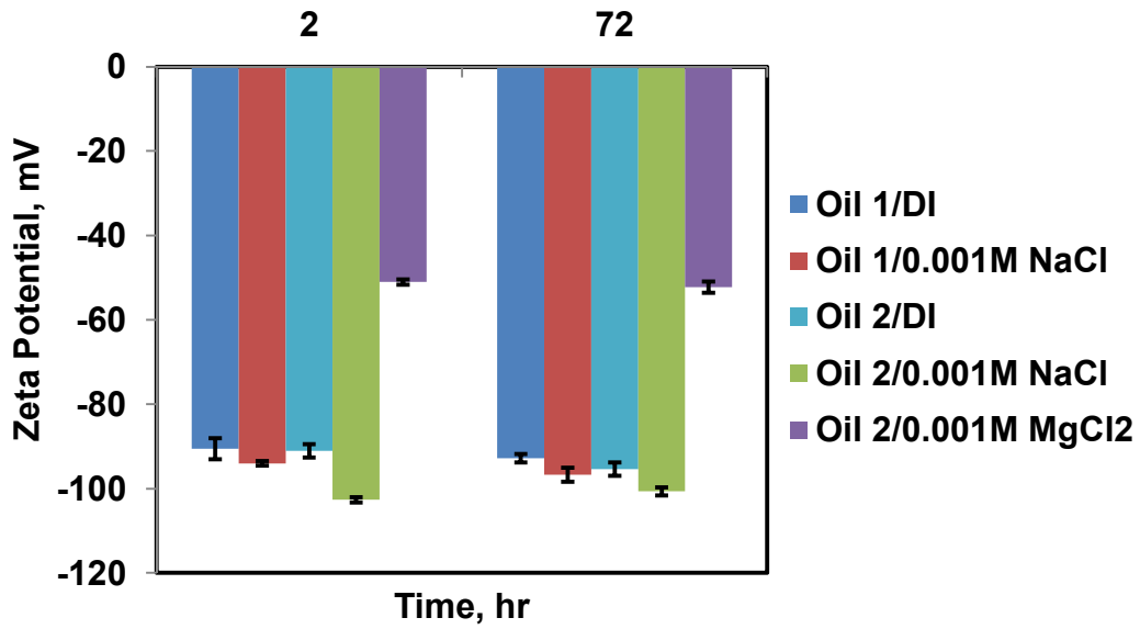
Figure 2: Effect of aging time on the zeta potential of Oil/Brine interfaces.
