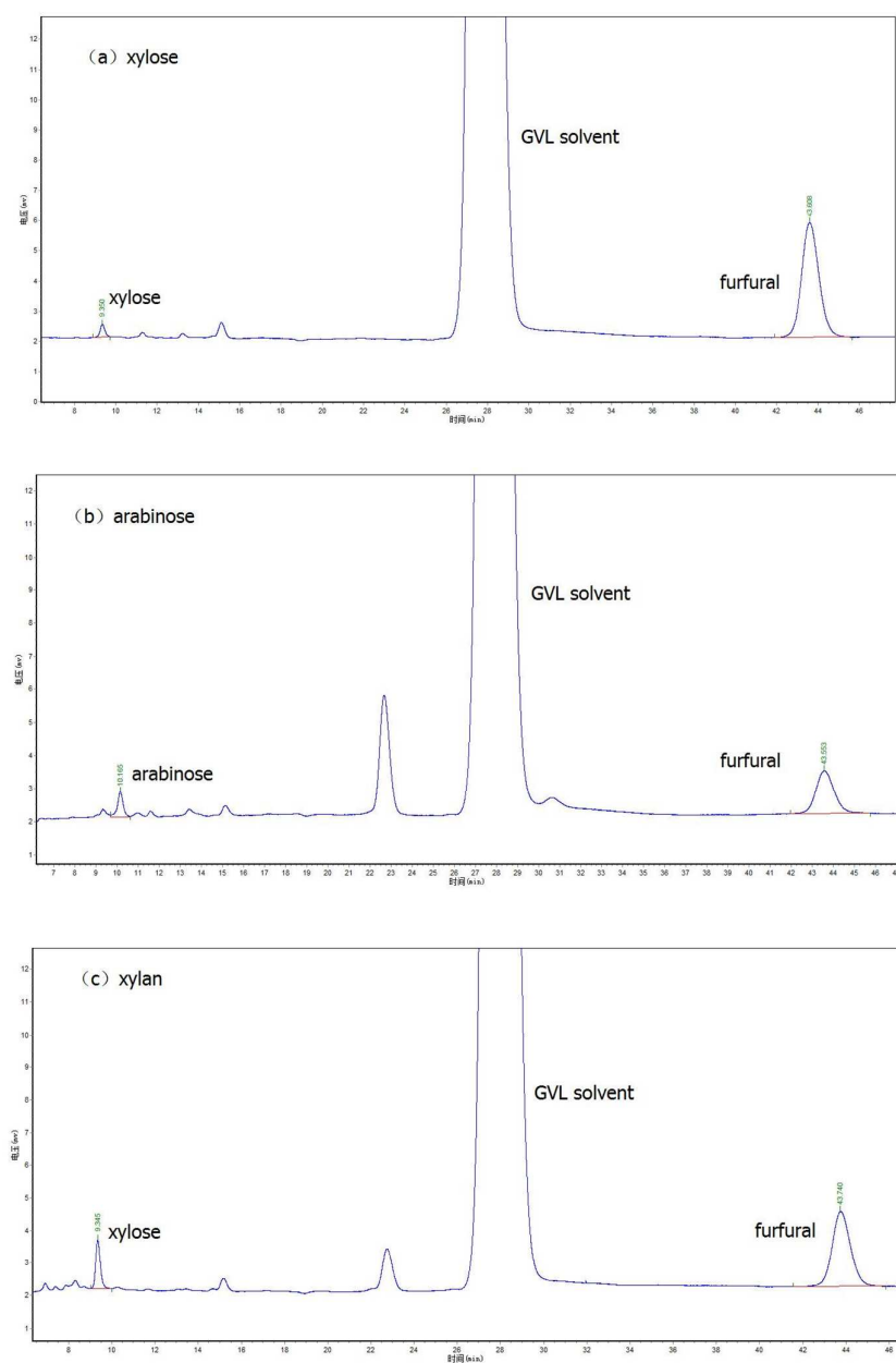
Fig. S1 Typical HPLC chromatographs of the product solution after the conversion of xylose (a), arabinose (b) and xylan (c). (140 °C, 180 min, water-GVL (1:19), 30 mg/ml substrate, 0.1 M IL1)
