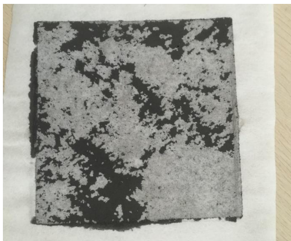
Figure S1 Free-standing LCO electrode sticking to filtration membrane with adding only 2% MWCNTs.
