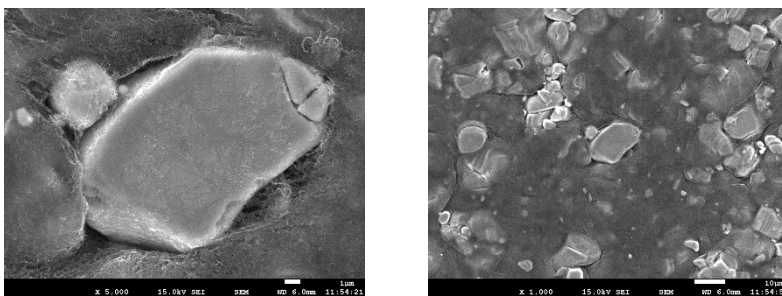
Figure 2. SEM of the electrode after cycling
