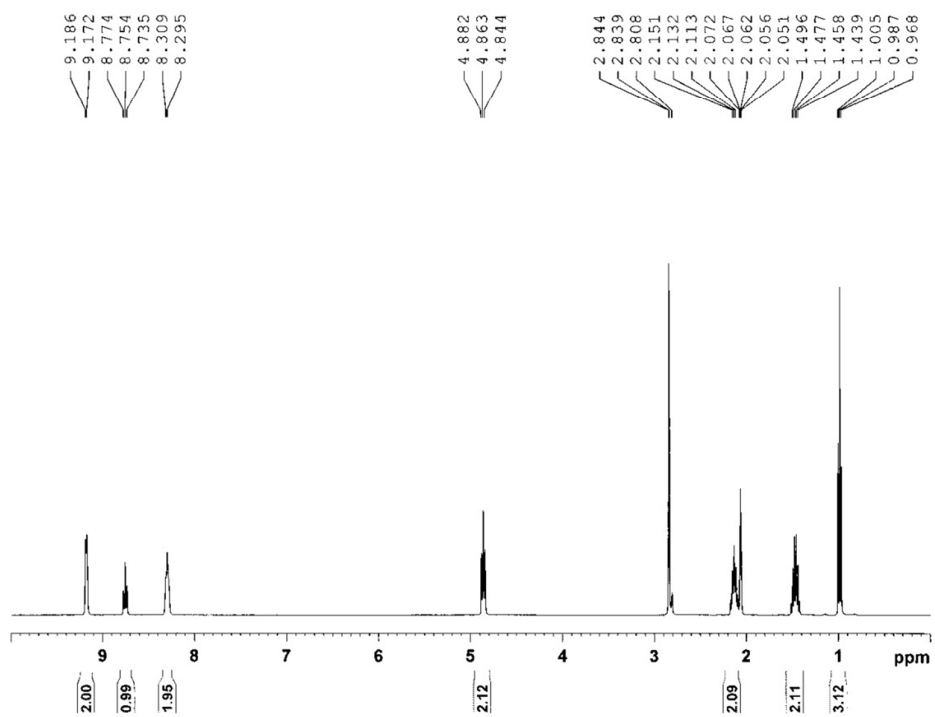
Figure S1. the NMR of ionic liquid [BPy] \text{NO}_3 (Deuterated acetone)
