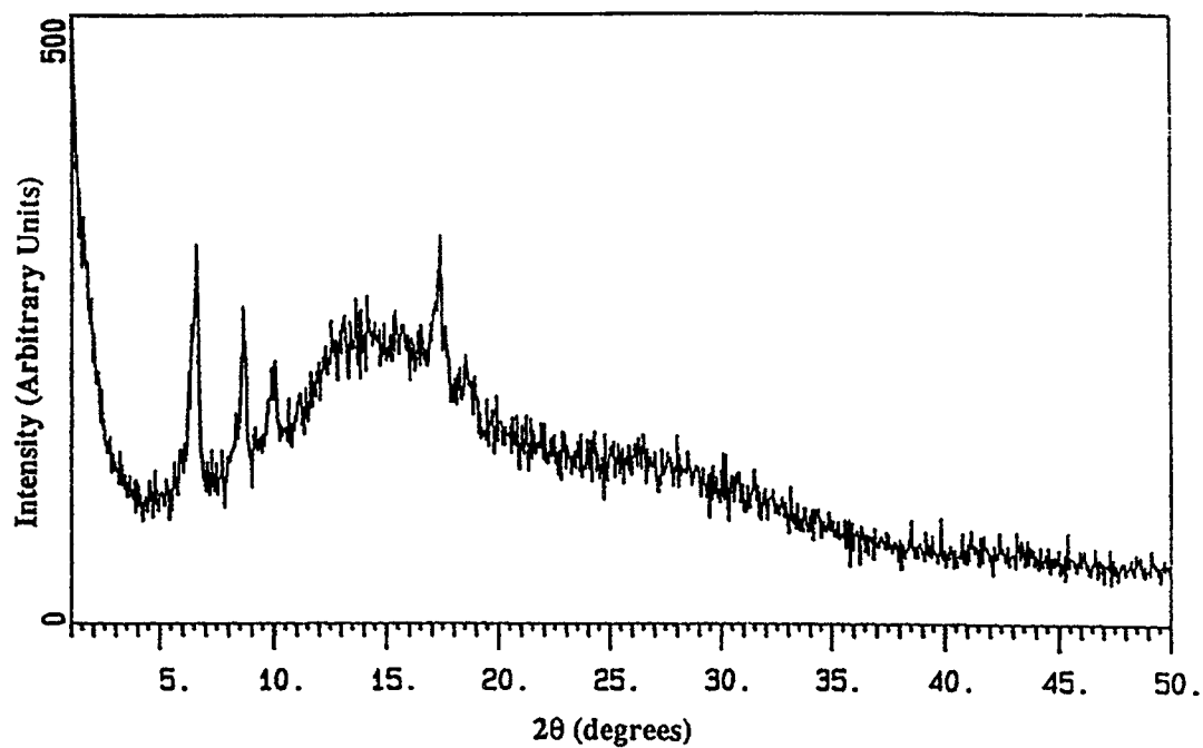
Supporting Figure 4. X-ray powder diffraction pattern recorded for a thin film of 20 wt% [Bu 2 Ph 2 Tth]PF 6 /PMMA.
