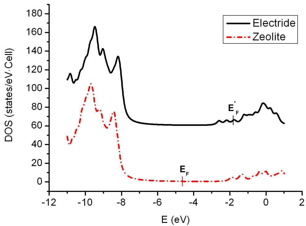
DOS of the inorganic electride and zeolite ITQ-4. The DOS are obtained by the \Gamma -only band structure calculations with a supercell (1x1x2). The Fermi levels are marked by short lines.
