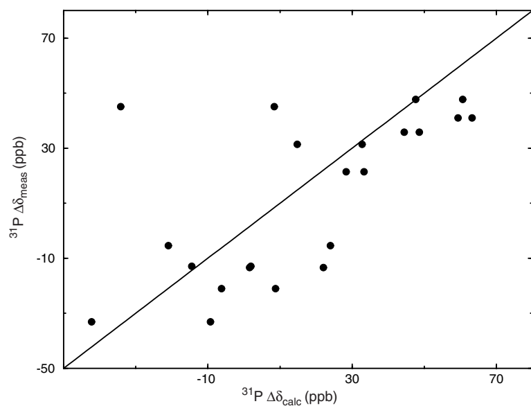
Supporting Information Figure 1. Correlation between observed \Delta\delta^{31}\text{P} values and those predicted by the 1BNA crystal structure of \text{d}(\text{CGCGAATTCGCG})_2 .
