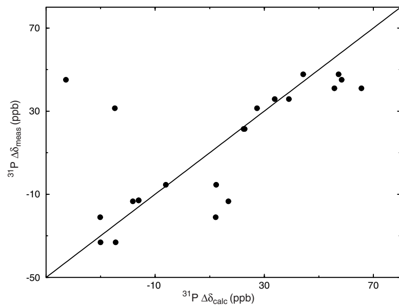
Supporting Information Figure 1. Correlation between observed \Delta\delta^{31}\text{P} values and those predicted by the 355D crystal structure of \text{d}(\text{CGCGAATTCGCG})_2 .
