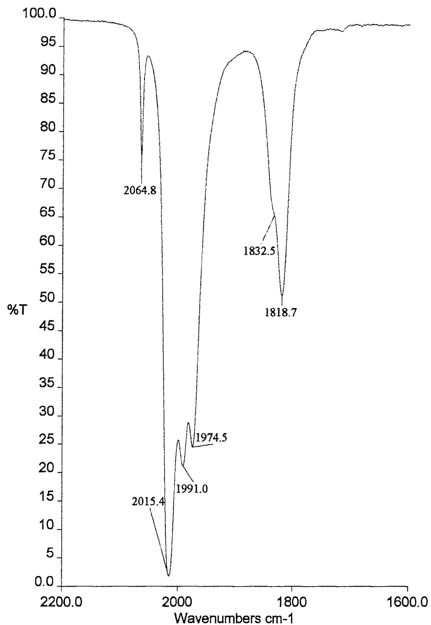
IR spectrum of [PPN][Ru 3 Rh(CO) 13 ] in THF
