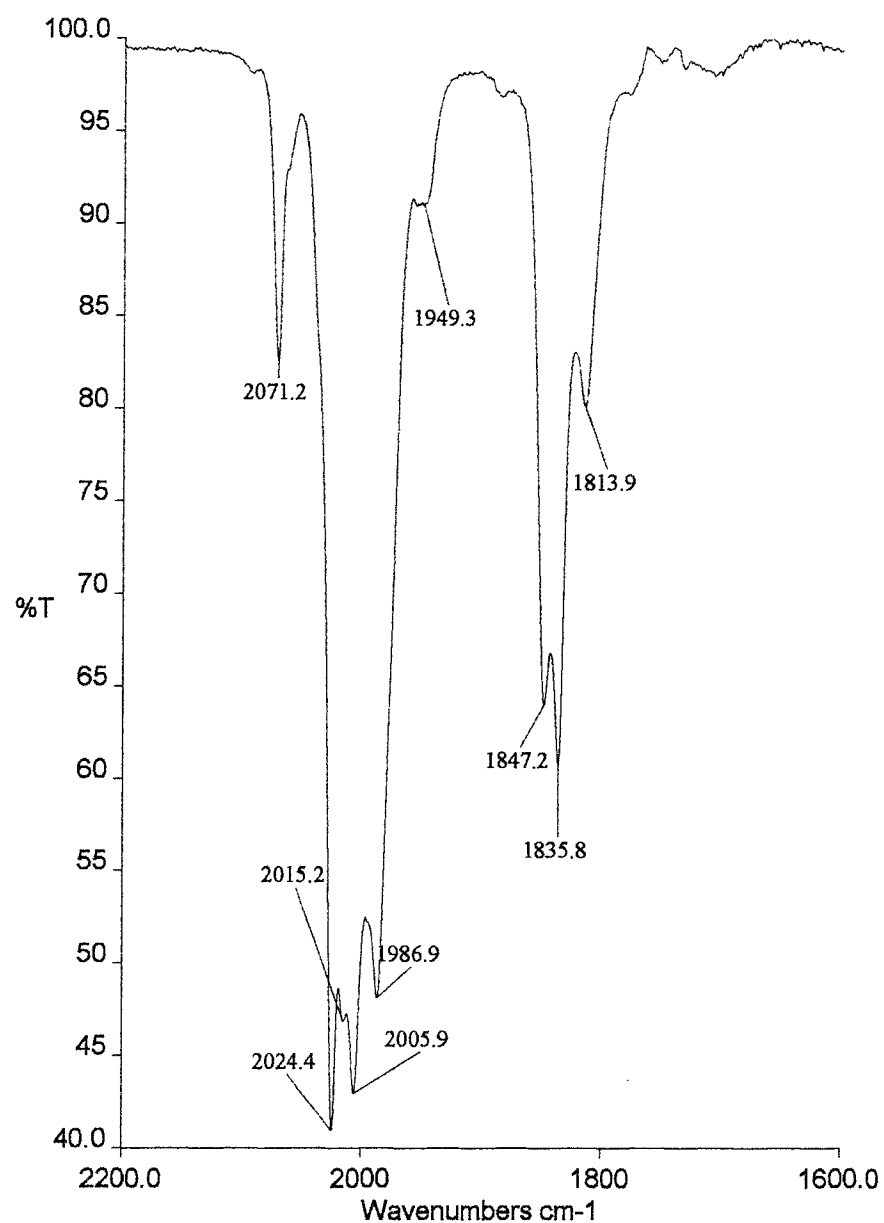
IR spectrum of [PPN][RuRh 3 (CO) 12 ] in THF
