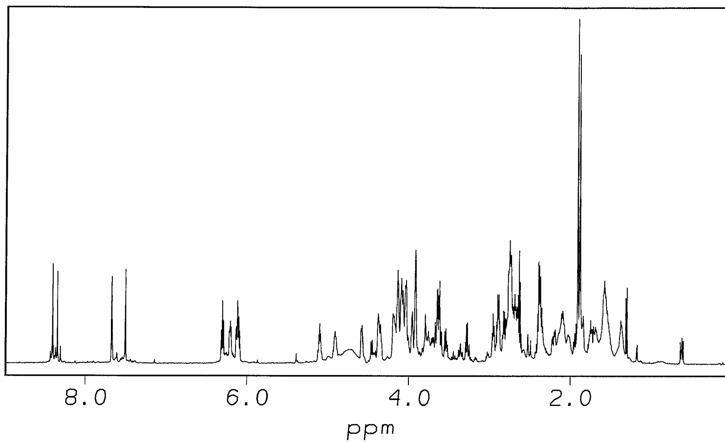
Figure S1: 1D ^1\text{H} NMR spectrum in \text{D}_2\text{O} of the d(TGGT) / bisPt-6 adduct ( 28^\circ\text{C} , pH 8.8)
