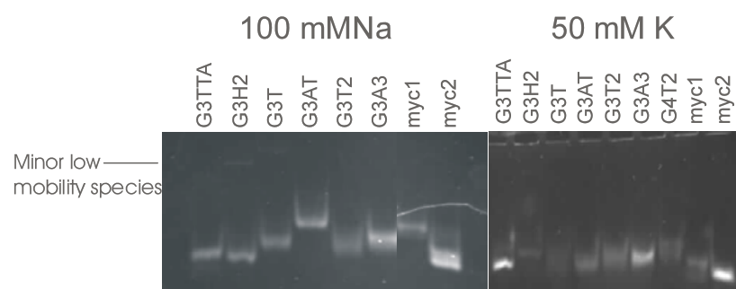
Figure 1. Mobility of the different DNA fragments on a 15% non-denaturing polyacrylamide gel, run in the presence of 100 mM Na or 50 mM K.
