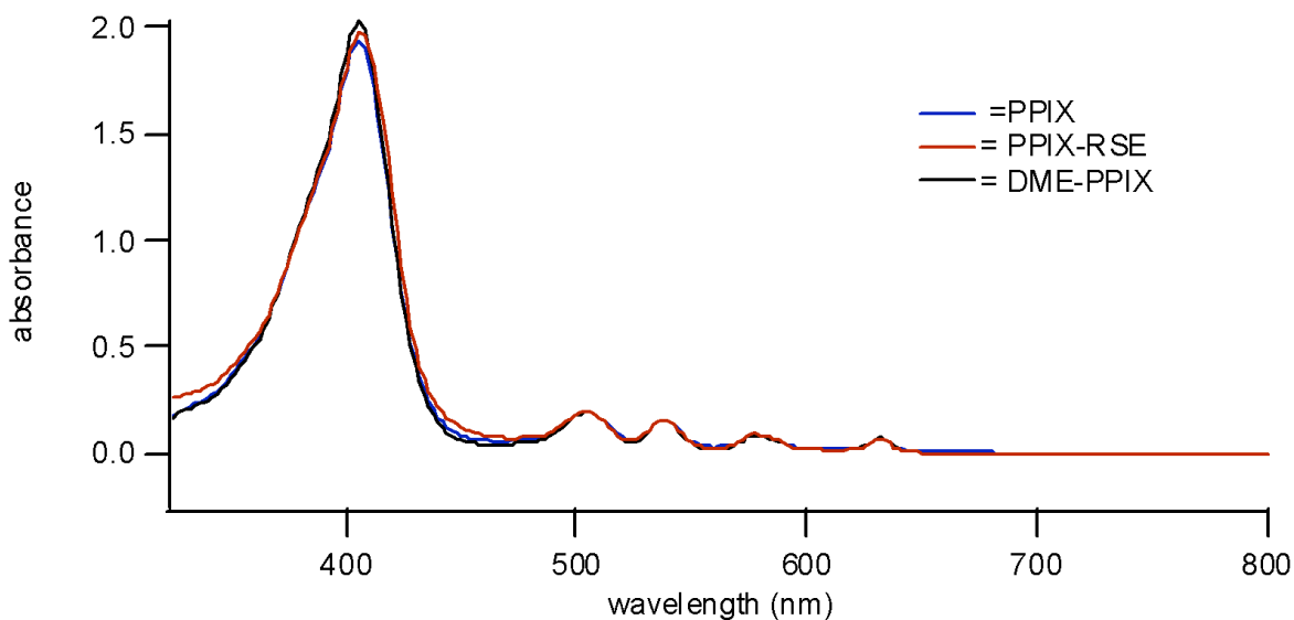
Figure S-1 (a) Electronic spectra of PPIX (13.5 \mu M), DME-PPIX (11.6 \mu M), and PPIX-RSE (13.3 \mu M) in tetrahydrofuran solution.
