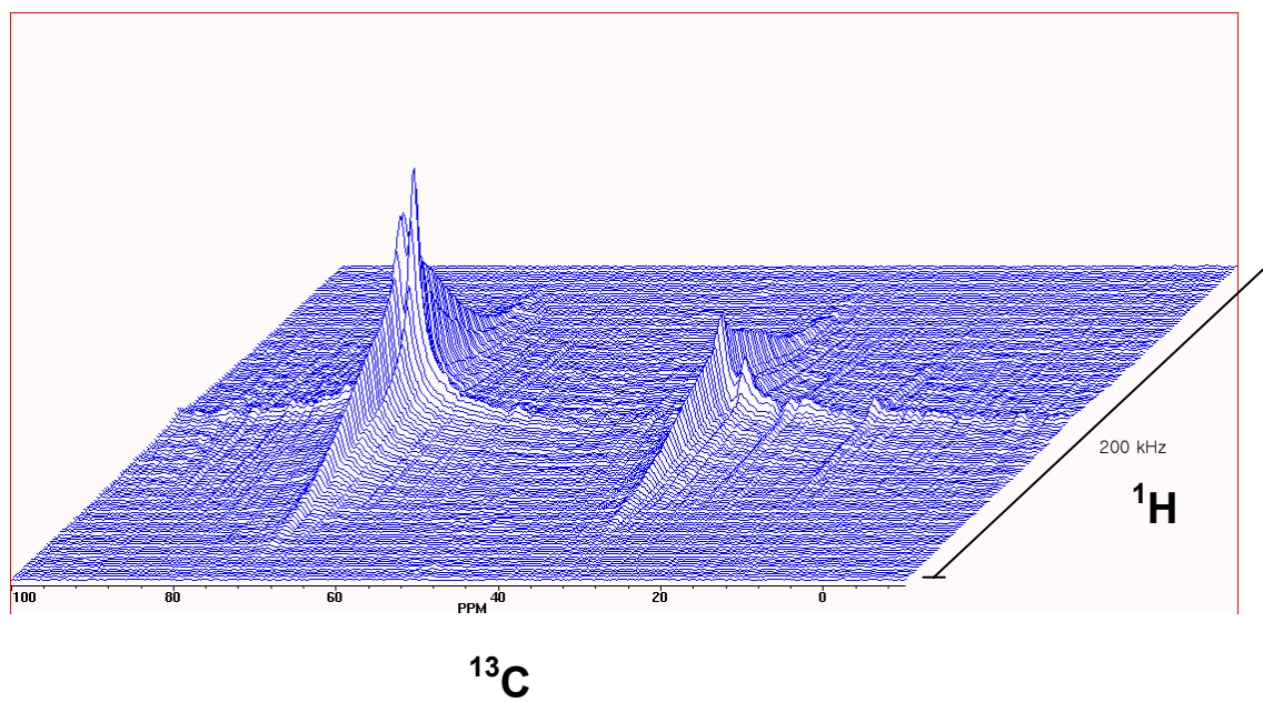
Figure B. 2D WISE NMR spectrum of HEUR 2(18) with the CP contact time of 1 ms.
