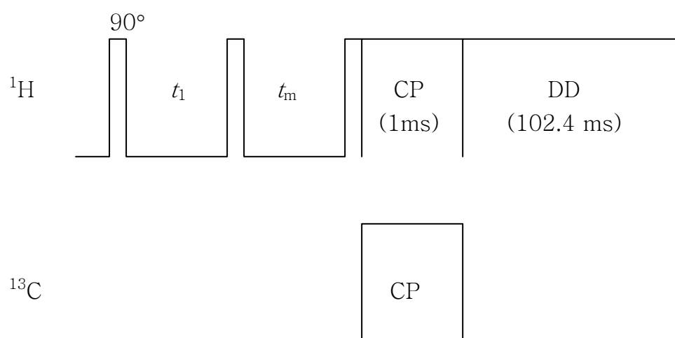
Figure A. Pulse sequence of 2D WISE NMR experiment. The cross polarization (CP) and ^{13}\text{C} acquisition with dipolar decoupling of protons (DD) are used as basic 1D CP experiment.
