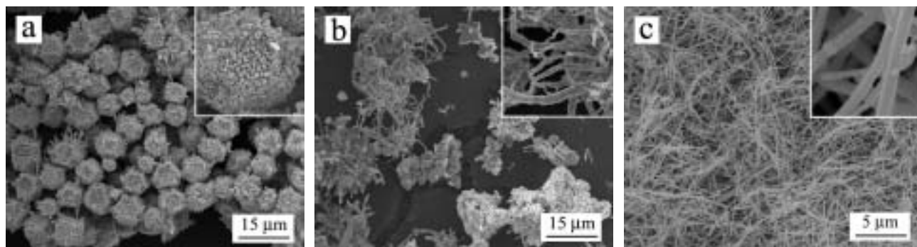
SI-Figure 1. FESEM images of three samples showing the variation of morphology when the concentration of SDBS was changed. (a) 0 mM; (b) 1.5 mM; (c) 9 mM. Other conditions were the same as those indicated in Figure 3. The local enlargement shows in the inset of each image.
