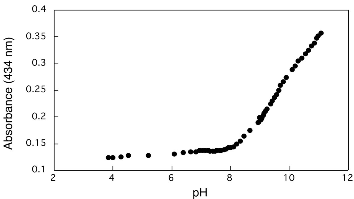
S2. pH-metric titration of Fusion-lip including 6a at 20°C.
