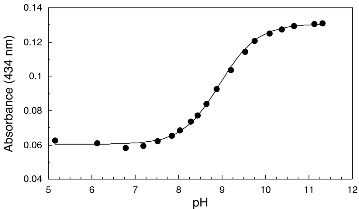
S1. pH-metric titration of Fusion-lip including 6b at 20°C.
