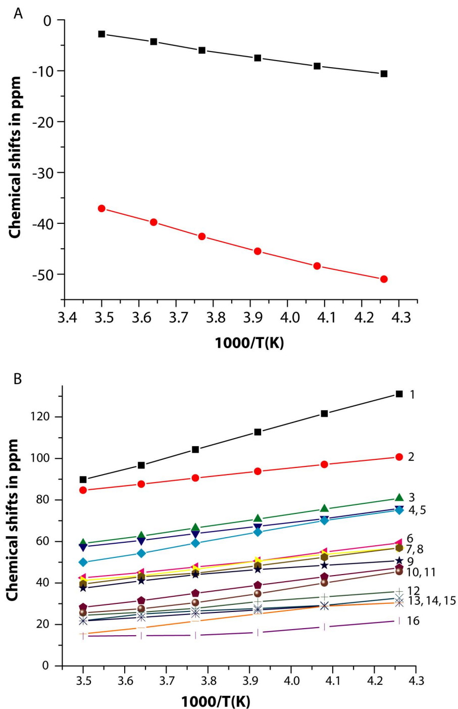
Figure S1. A plot of chemical shift versus 1/T for the open-chain tetrapyrrole complex 3 . Meso resonances are plotted in the top part while the methylene resonances are shown in the lower portion.
