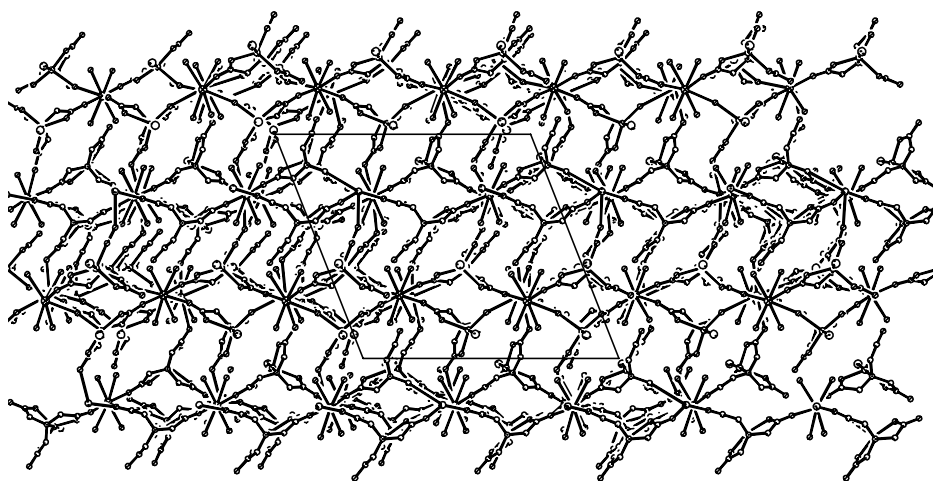
S2. Two-dimensional layered molecular structure of 1 , 2 and 3 . The alkaline metal ions are omitted for clarity.
