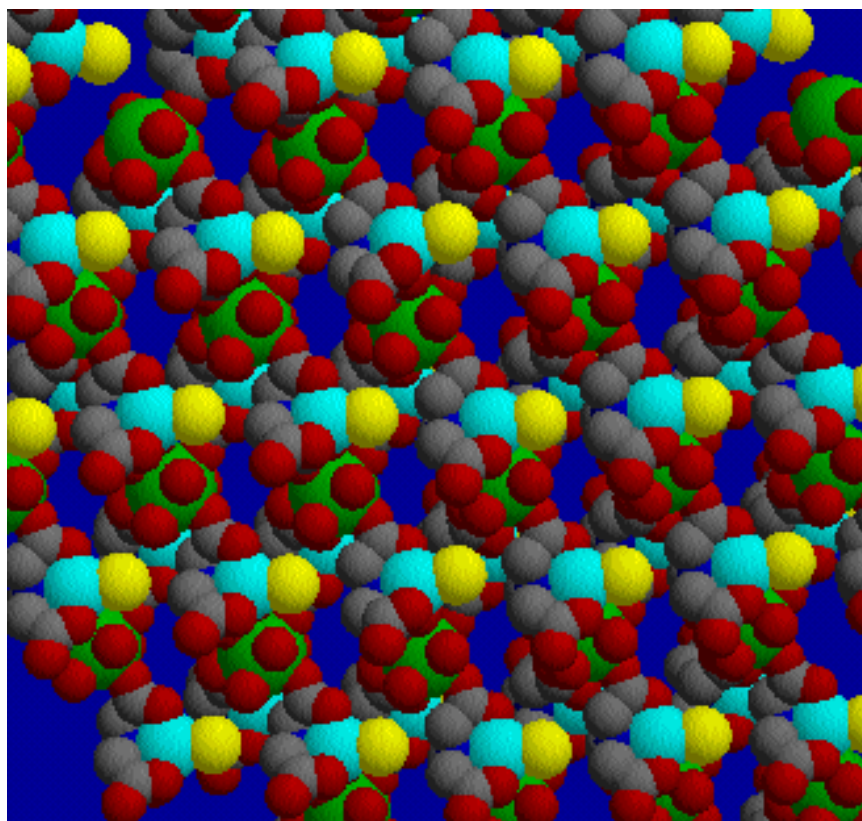
S1. Space-filling diagram showing the cavities. Cl yellow, Gd green, N blue, Cu turquoise
