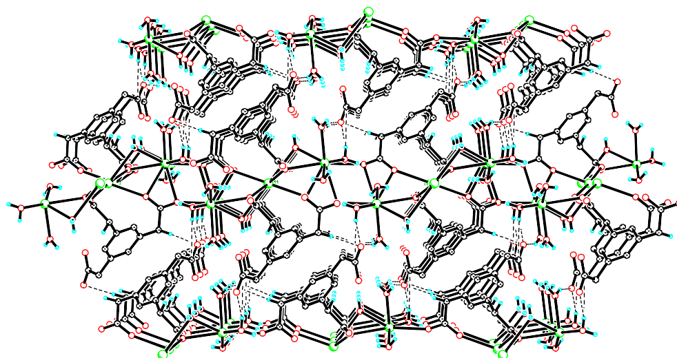
Figure S3 Crystal packing diagram for 2 with hydrogen bonds indicated by dashed lines.
