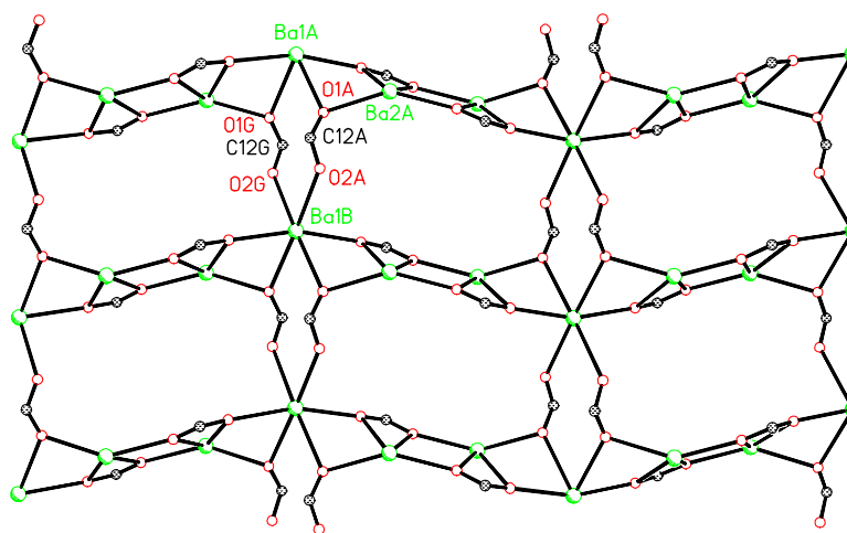
Figure S2 Ba-O wave-like chains of 2 linked by \text{-COO}^- to form a 2D structure.
