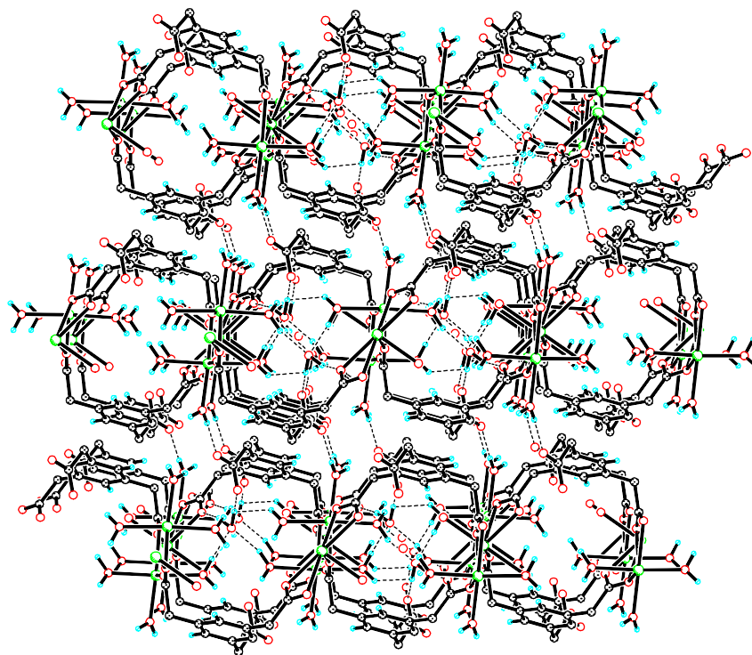
Figure S1 Crystal packing diagram for 1 with hydrogen bonds indicated by dashed lines.
