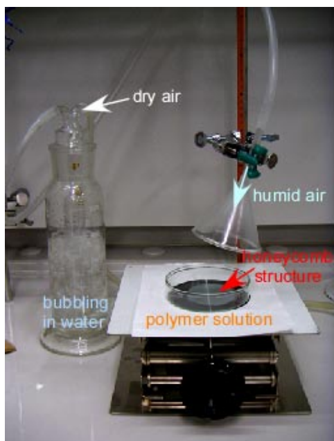
Figure S1: Experimental set up of preparation of honeycomb-patterned films. The experiment was performed under moderate conditions.
