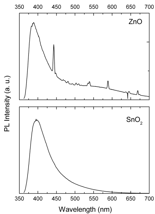
Figure S3: PL spectra measured on diluted ZnO and SnO 2 suspensions.
