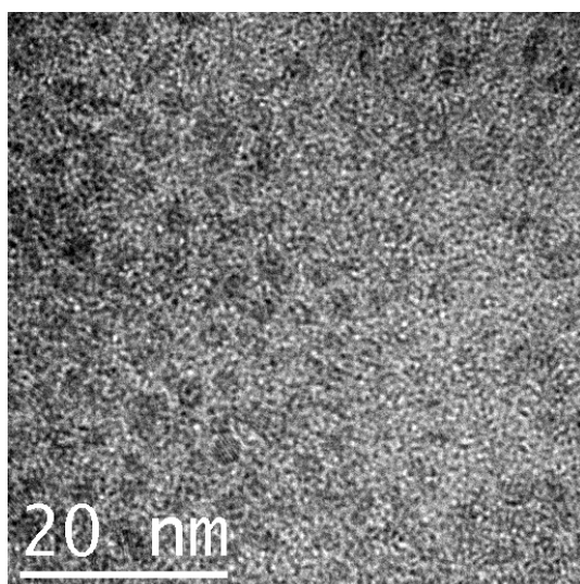
Figure S2: Bright field TEM general view of SnO 2 nanocrystals.
