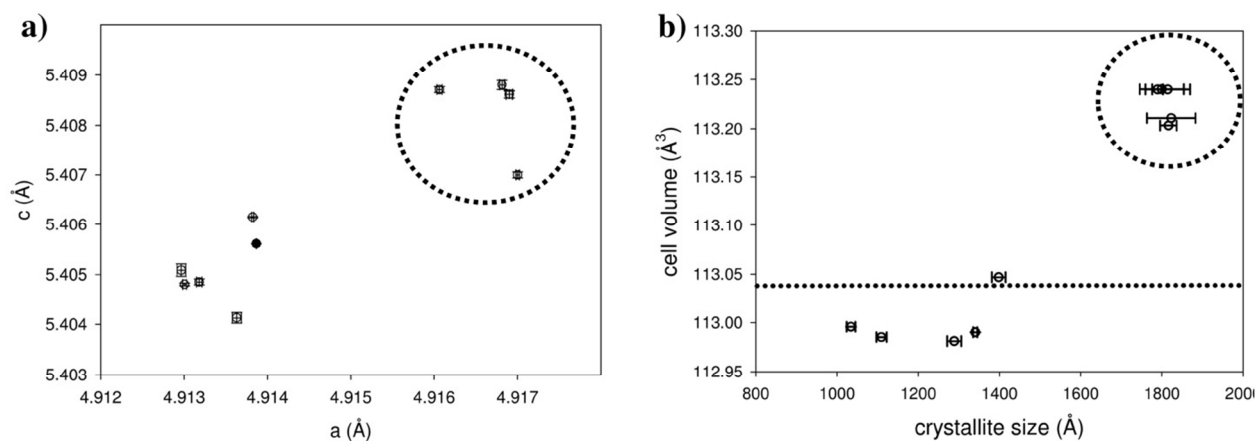
Figure S1. Comparison between the cell parameters (a), and the cell volume and crystallite size (b) of NG and CG (inside the dotted circle) crystals, as calculated by Rietveld refinement. The black point and the line represent the dimensional parameters of the SRM 1878a standard quartz sample.
