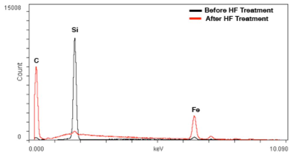
Supplementary Figure 1: A) EDS data for MWNT-silica membrane before and after HF treatment. B) EDS data for the multilayered MWNT-silica structure before and after HF treatment.
