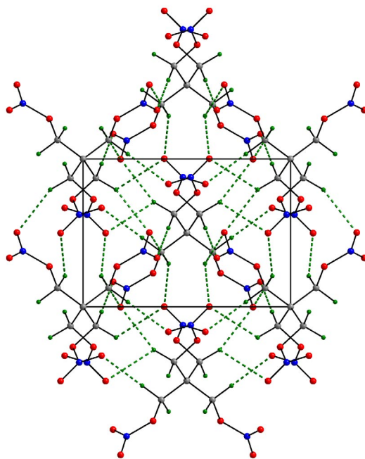
PETN packing diagram showing hydrogen bonds as green dashed lines – projection down the a-axis.
