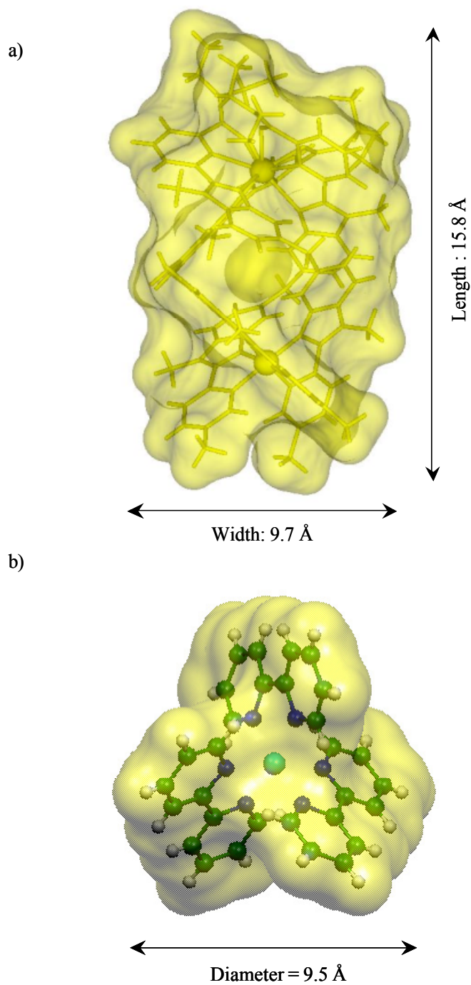
Figure S1 Crystal structures of a) [\text{RuLu}(\text{L5})_3]^{5+} 11 and b) [\text{Ru}(\text{bipy})_3]^{2+} 27 with Connolly surfaces. 26
