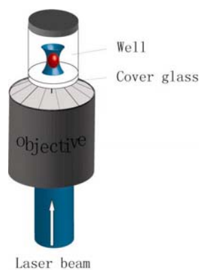
Figure S-1. The schematic diagram of small well used for detection chamber of FCS experiments.
