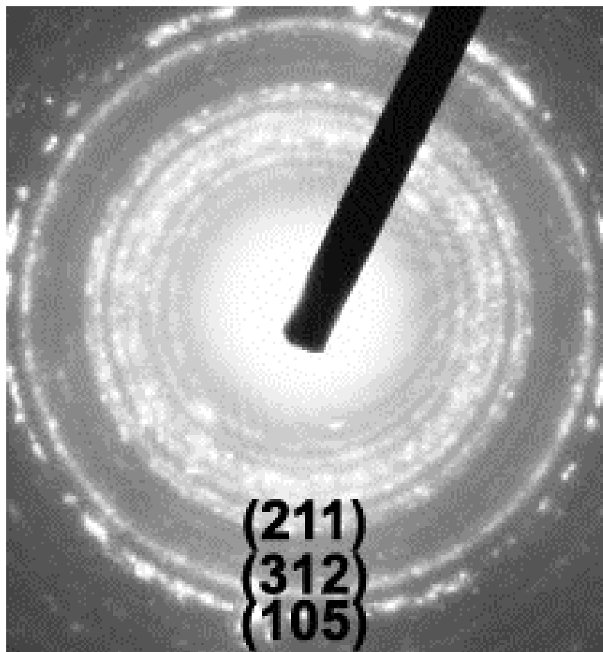
Figure S2. Electronic diffraction pattern of the BaCu 2 S 2 thin film
