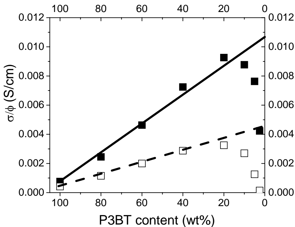
Figure S2. Dependence of \sigma/\phi of P3BT/PMMA composite on P3BT content ( \phi ) in the composites as measured with 4-probe method (solid square) and 2-probe method (open square), respectively.
