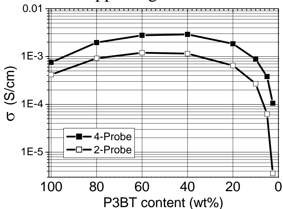
Figure S1. Dependence of P3BT/PMMA conductivity on P3BT content in the composites as measured with 4-probe method (solid square) and 2-probe method (open square), respectively.
