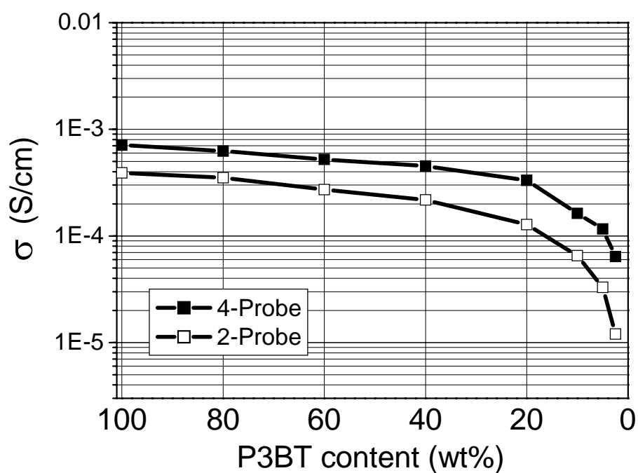
Figure S3. Dependence of P3BT/regionrandom P3HT (RRa-P3HT) conductivity on P3BT content in the composites as measured with 4-probe method (solid square) and 2-probe method (open square), respectively.
