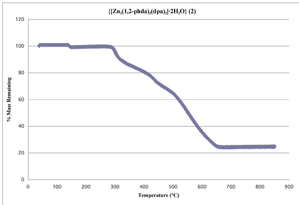
Figure S2. TGA trace for 2 .
