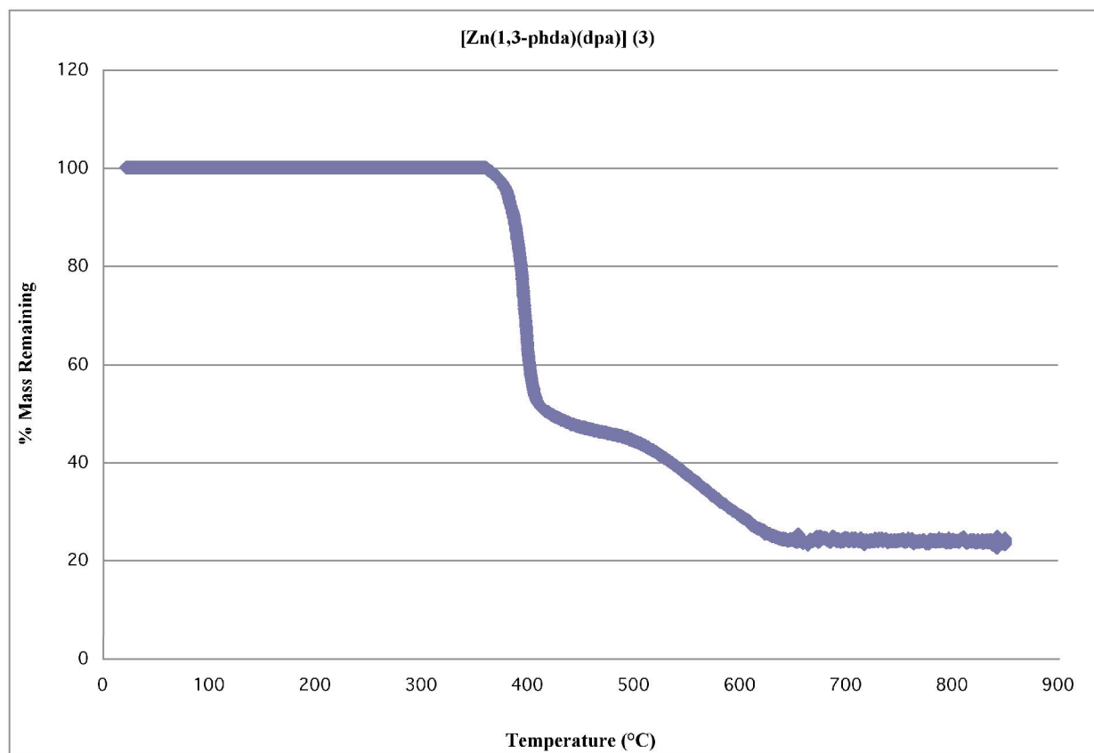
Figure S3. TGA trace for 3 .
