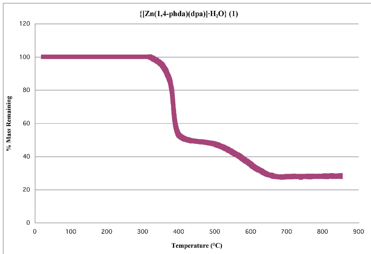
Figure S1. TGA trace for 1 .
