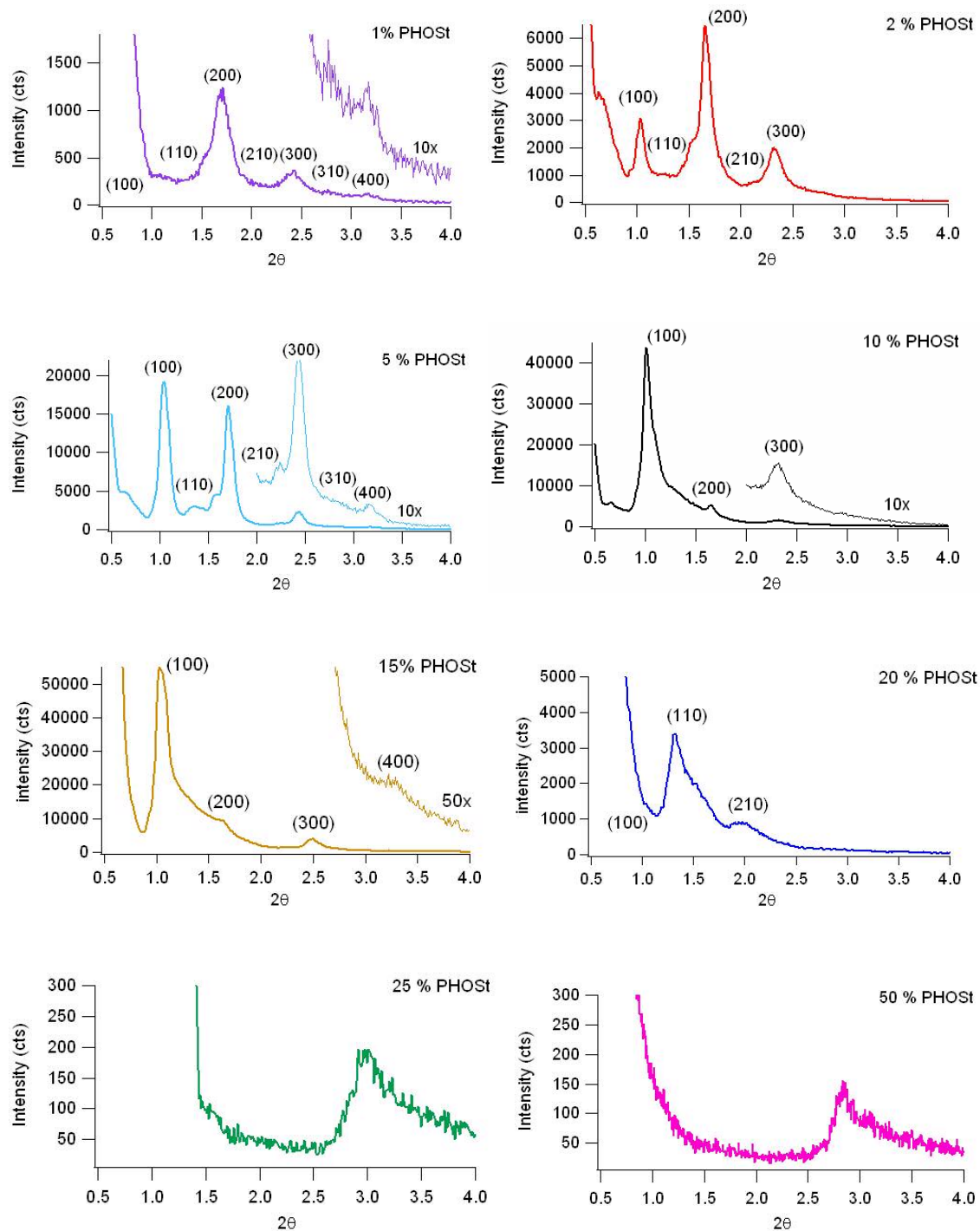
Figure S1. Individual X-ray diffraction profiles for calcined silica films as a function template composition. The reflection planes are identified for each profile where appropriate. For film FP1, FP2, and FP5, all the allowed planes for hexagonal P6mm are shown. For film FP10 and FP15, only (100), (200), (300)...are shown indicating significant orientation of the mesopores.
