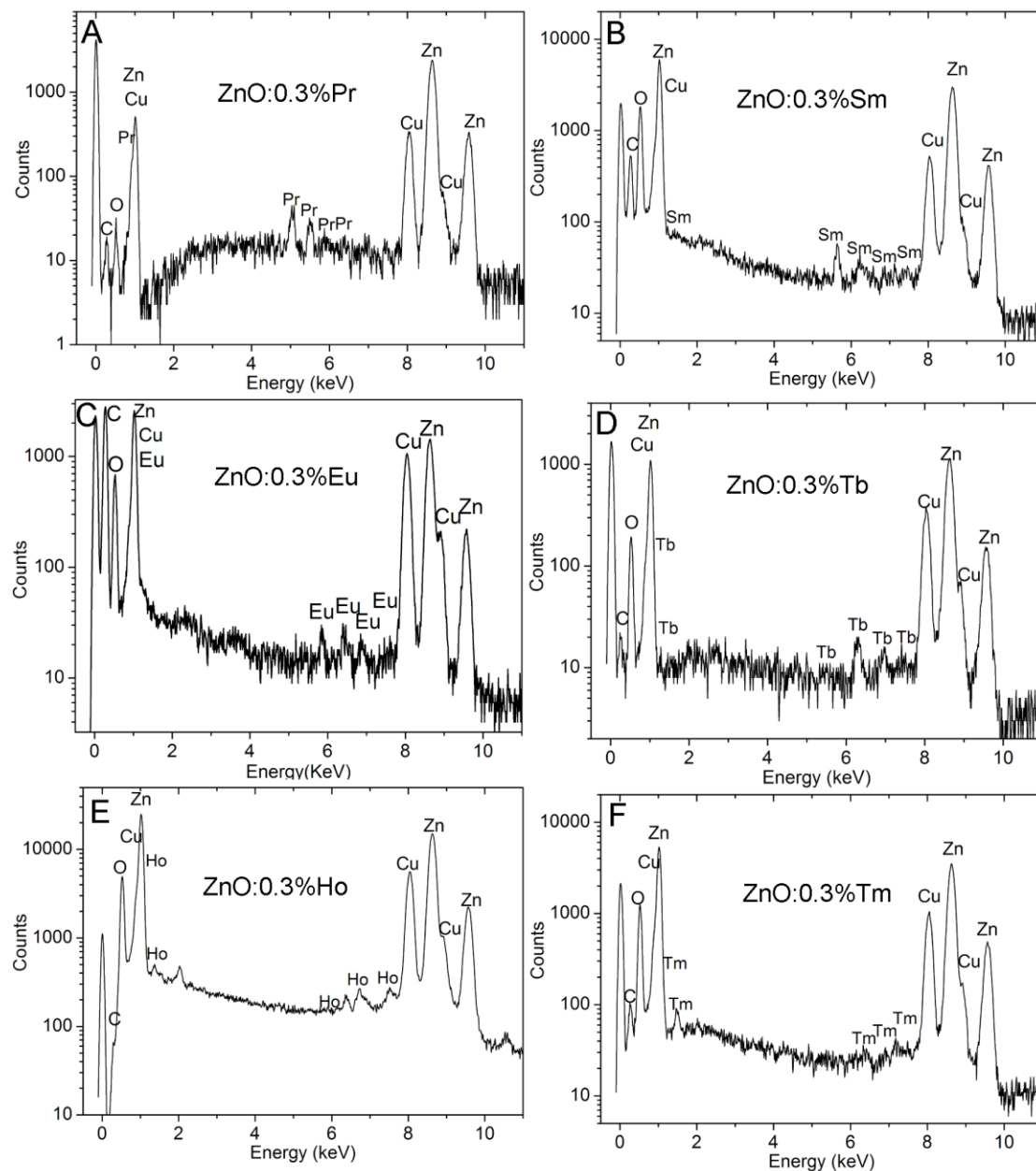
Figure S1. Typical energy dispersive X-ray (EDX) spectra of single ZnO:RE (RE=Pr, Sm, Eu, Tb, Ho, Tm) nanosheet. The signals were recorded on the transmission electron microscope (TEM, JEOL 2010, 200kV).
