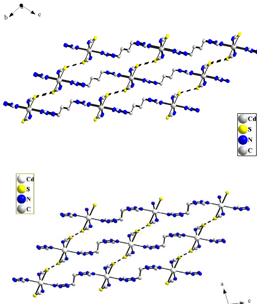
Figure S2. 3-D networks of 2 along b (up) and c (down) axis.
