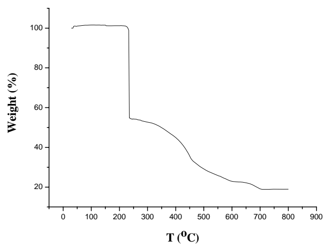
Figure S5. TG curve of 5 .
