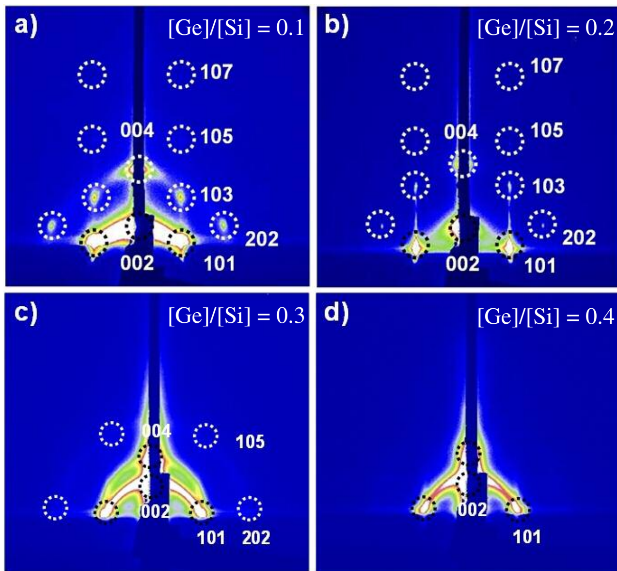
Fig. S1. Grazing incidence small-angle X-ray scattering patterns referring to sample SG1 (a), SG2 (b), SG3 (c) and SG4 (d) thermally treated at 100°C.
