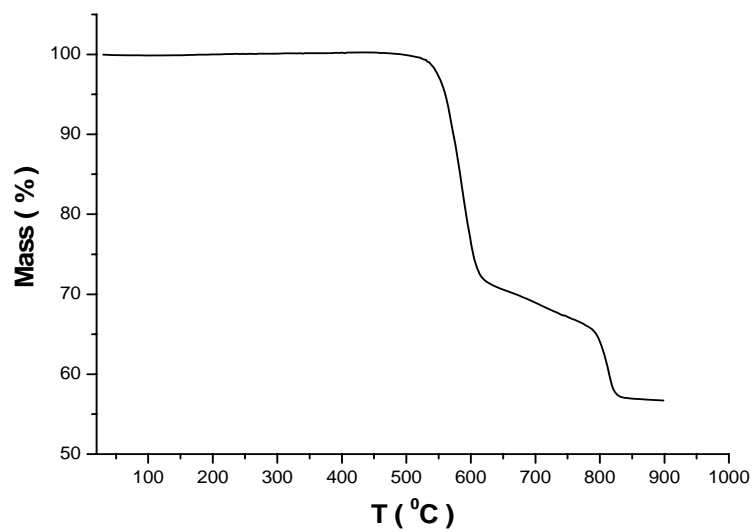
Figure 1. Thermogravimetric analysis for 1.
