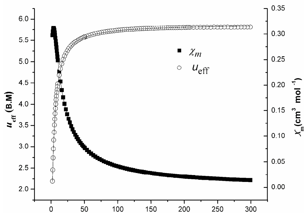
Figure S1. Plots of \mu_{\text{eff}} (○) and \chi_m (■) vs. temperature for 2 ; the solid line represents the best fit.
