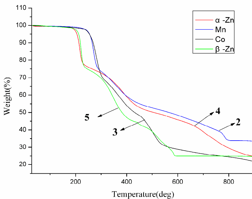
Figure S2 TGA showing the weight loss of compounds 2 (blue), 3 (black), 4 (red), 5 (green).
