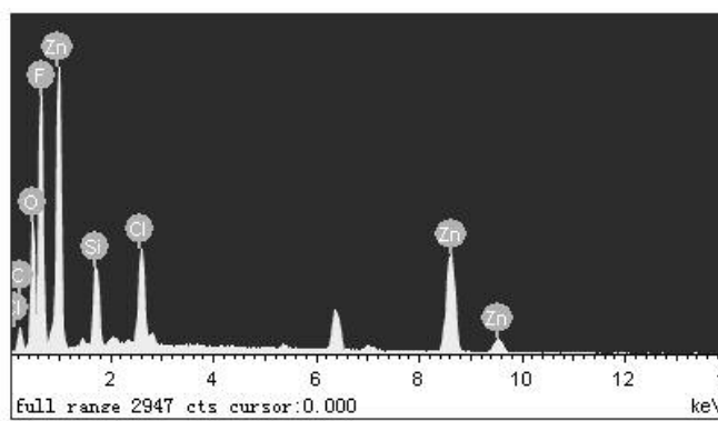
Figure S1. The EDX spectrum of the distributed elements for the superhydrophobic film on galvanized iron substrate.
