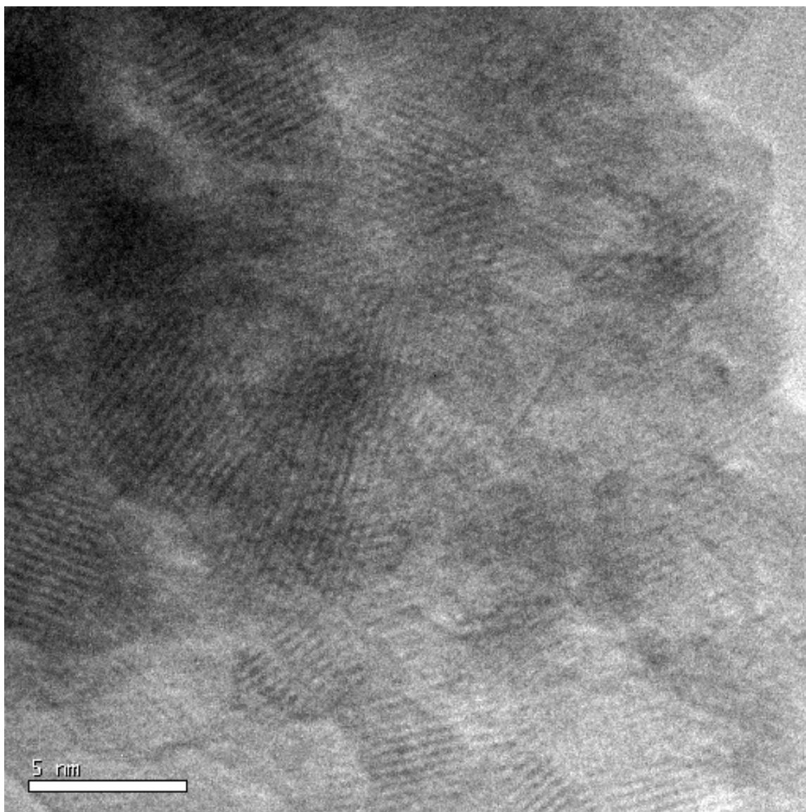
Figure S1. HR TEM image of the mesoporous anatase TiO 2 sample prepared by hydrolytic condensation of TiOB/EA, after calcinations at 400 °C.
