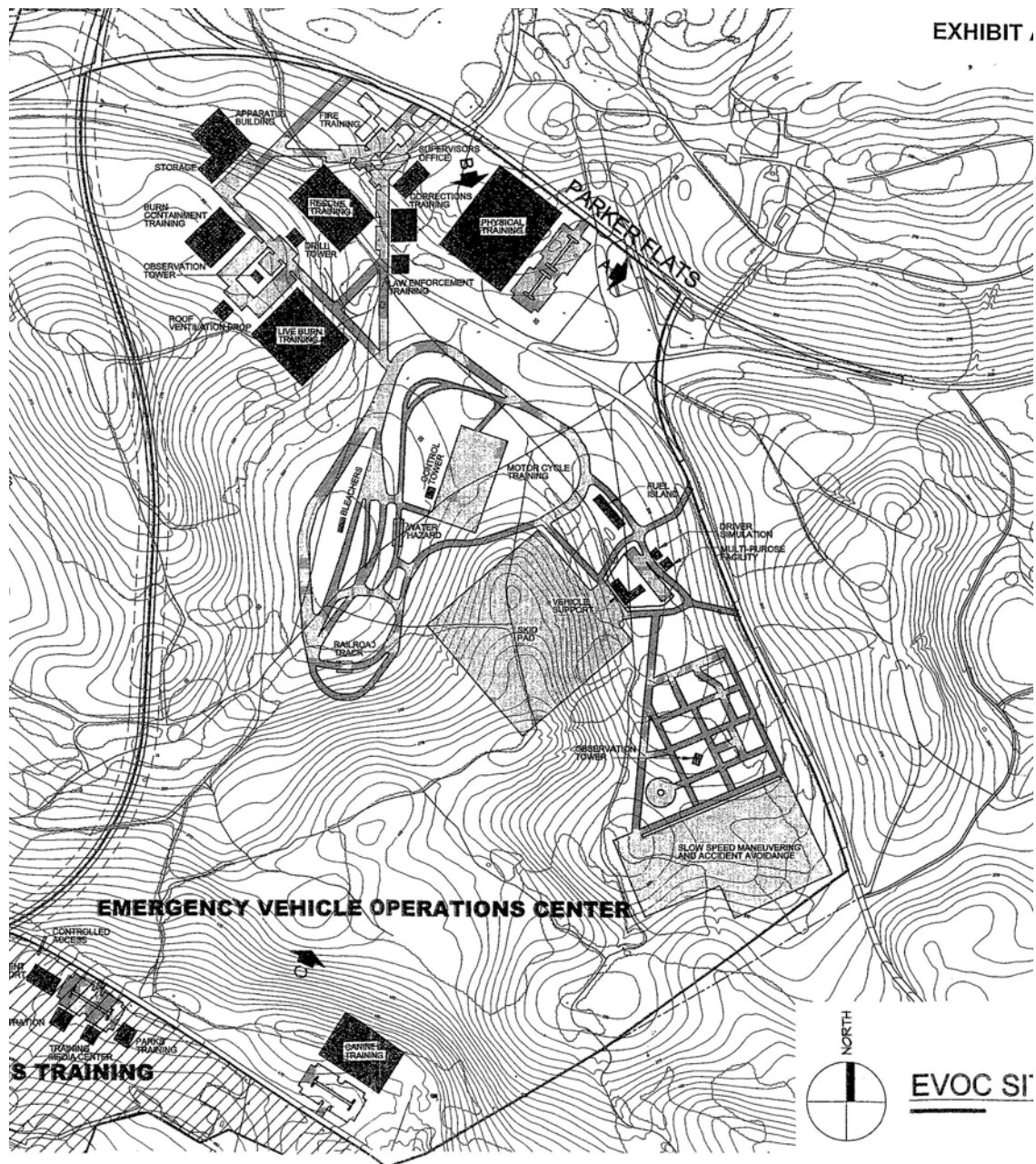
FIGURE SI 1 Plan for Monterey Peninsula College Emergency Vehicle Operations Center, to be constructed at Fort Ord Site OE-53.
