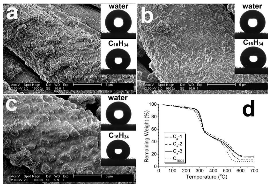
Figure S1. The morphology of C a samples: (a) C a -1 (b) C a -2 (c) C a -3, and (d) weight loss for the cotton textile samples (C a series) before and after each step of the modification by TGA. Shown in the inserts are the images of static water droplets (5 μL) and C 16 H 34 droplets (5 μL) on the respective textiles modified by Rf-Si, namely (a) C a -1-Rf, (b) C a -2-Rf, and (c) C a -3-Rf.
