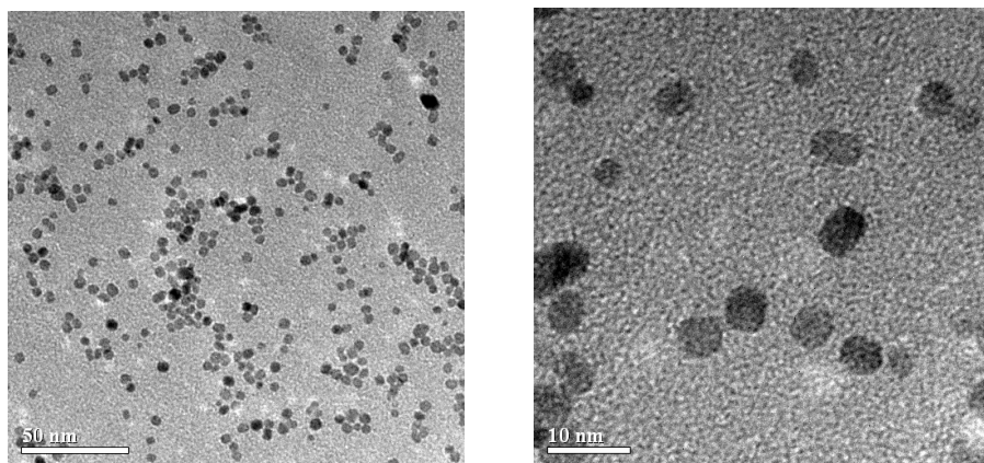
Figure 1. TEM micrographs of Pd nanoparticles
