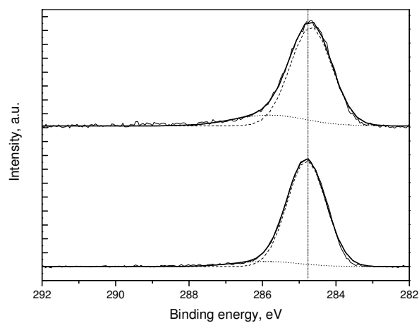
Figure 2. Carbon XPS spectra of Au/HDT monolayer (bottom) and Au/HDT/Pd (top). Fitted peaks of C 1s and its oxidized form are represented by dashed and dotted lines respectively.
