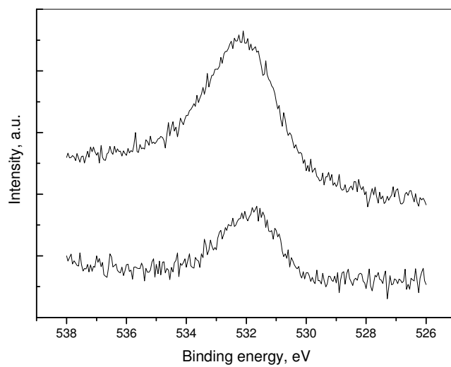
Figure 3. Oxygen XPS spectra of Au/HDT monolayer (bottom) and Au/HDT/Pd (top).
