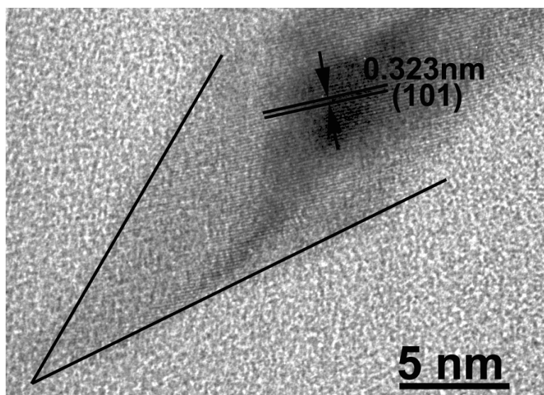
Figure S1. Enlarged HRTEM image of inset Figure 3d of the tip of the Te nanoneedles.
