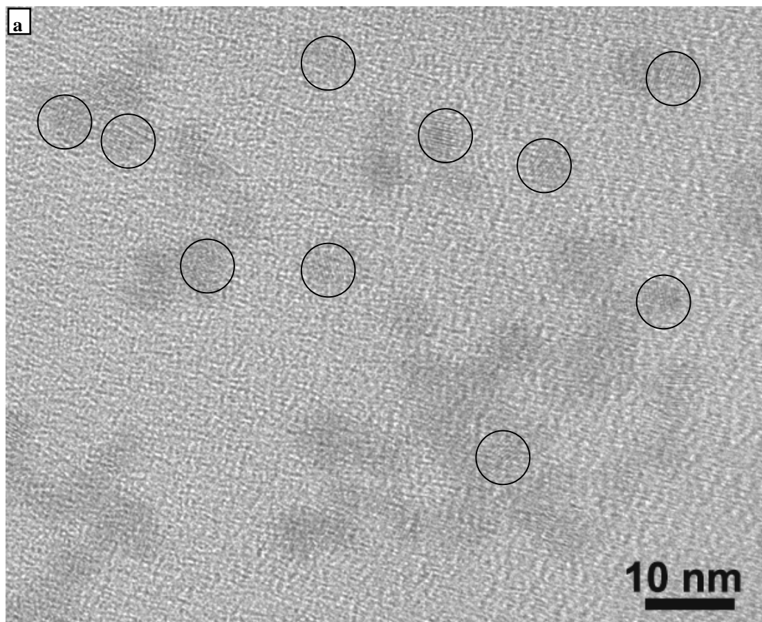
Figure S2. Enlarged HRTEM image of Figure 5a of the CdTe nanocrystals.
