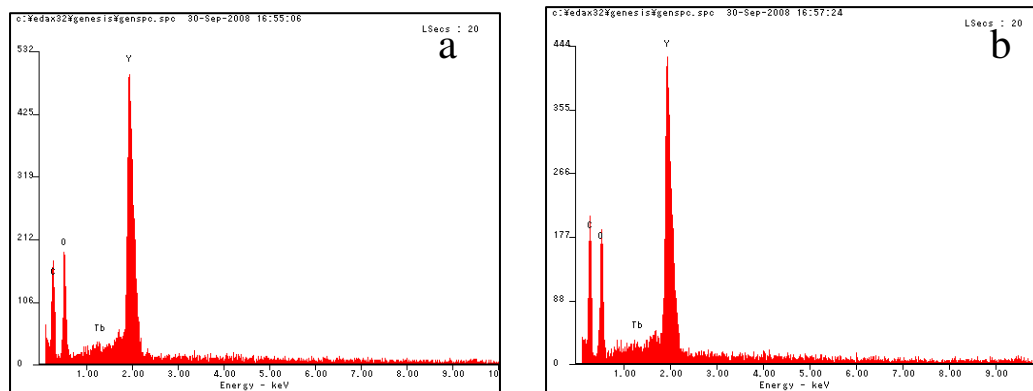
Figure S1. EDS spectra of as prepared precursor sample (a), and calcined samples at 900°C for 4 h (b).
