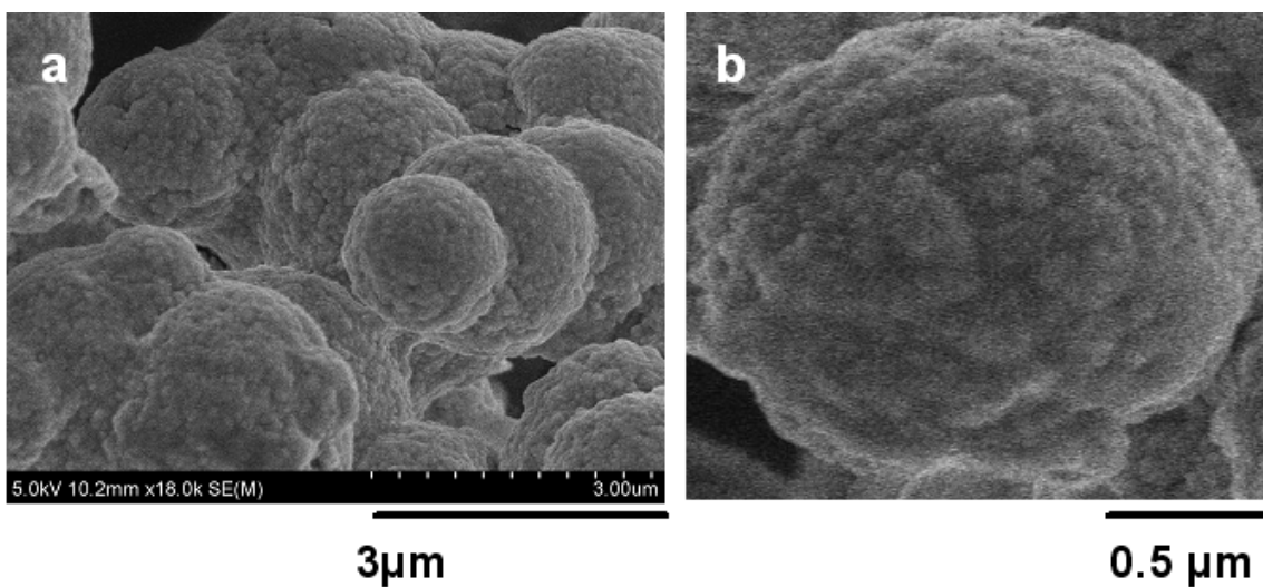
Figure S2. FESEM image of calcined sample at 1000°C for 4 h, showing many hollow microsphere (a), and single hollow microsphere (b).
