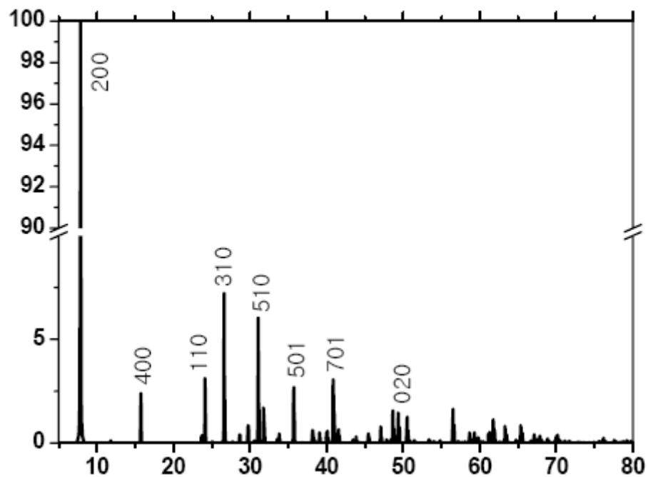
Simulated XRD pattern in Figure 2.
