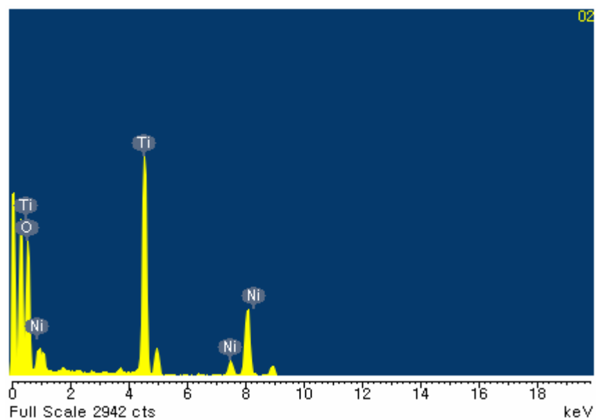
EDS spectrum of Ni doped nanotubes
