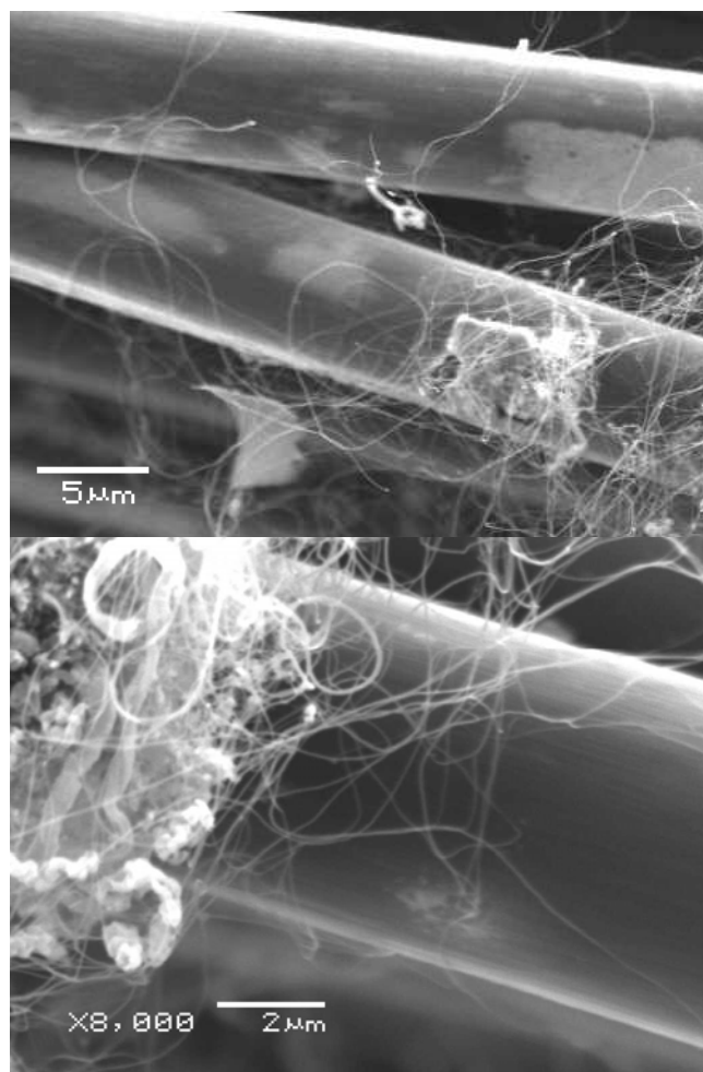
Figure S1. Long CNTs, CNT bundles, and large-diameter fibrils extending from a carbon fiber coated with zirconia nanoparticles produced by dip-coating in \text{ZrOCl}_2 solution followed by \text{H}_2 reduction.
