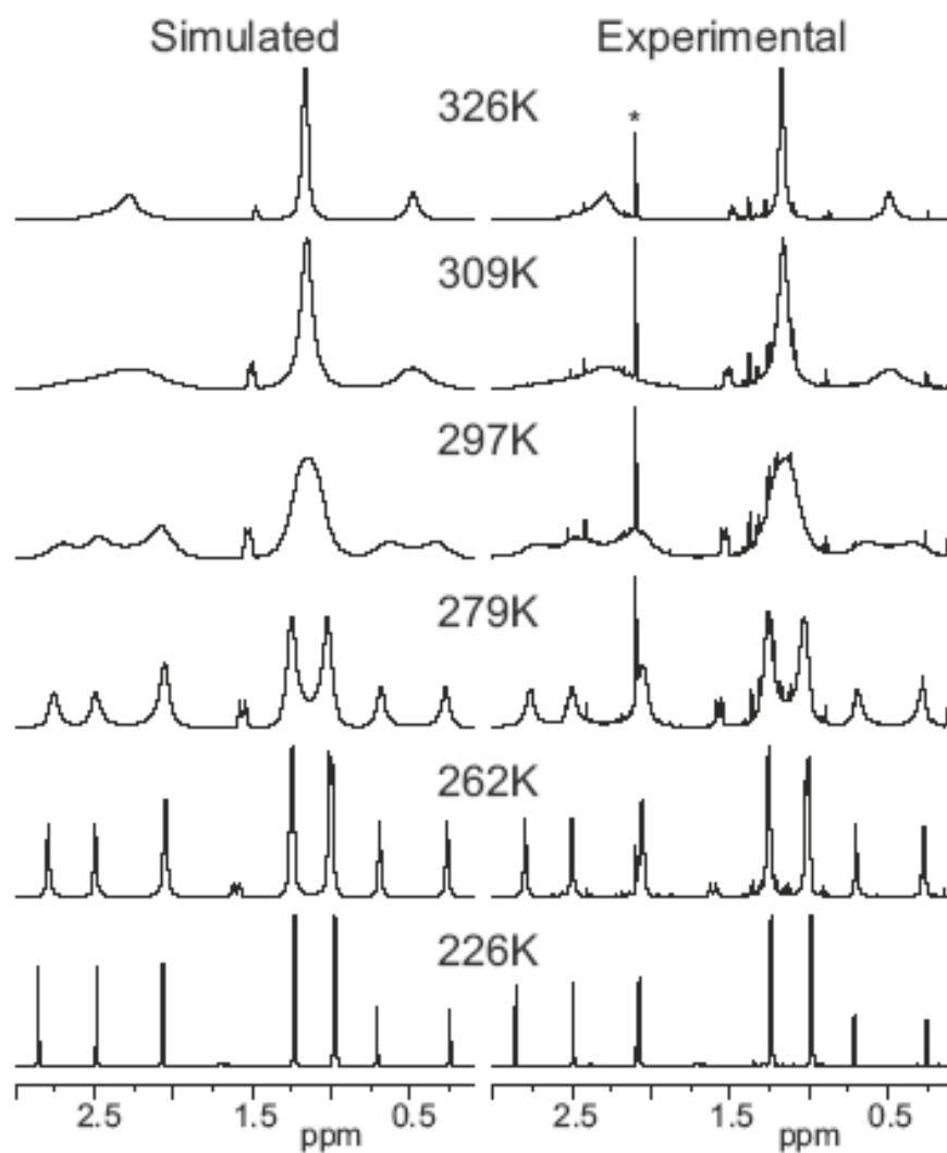
Figure SI1. Experimental (right) and simulated (left) VT 1 H NMR spectra for the degenerate exchange in compound 3c .
