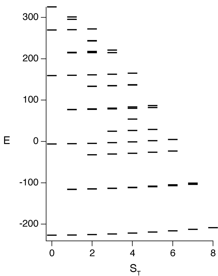
Figure S1. Energy level diagram for 1 .
