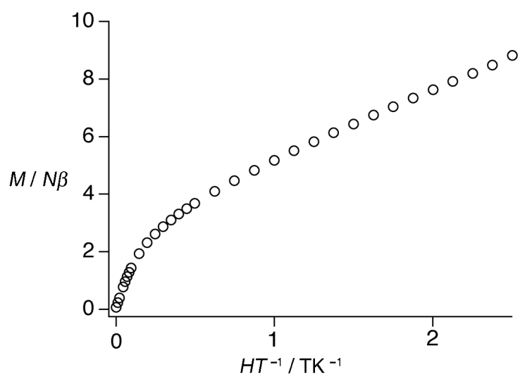
Figure S2. Field dependent magnetization for 1 at 2 K.
