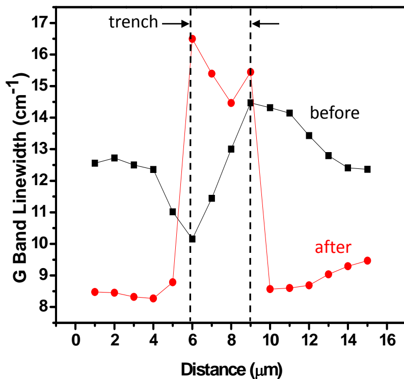
Figure 1. Spatial mapping of the G band Raman linewidth of the suspended graphene sample shown in Figure 1 of the manuscript taken before and after thermal cycling to 700K.
